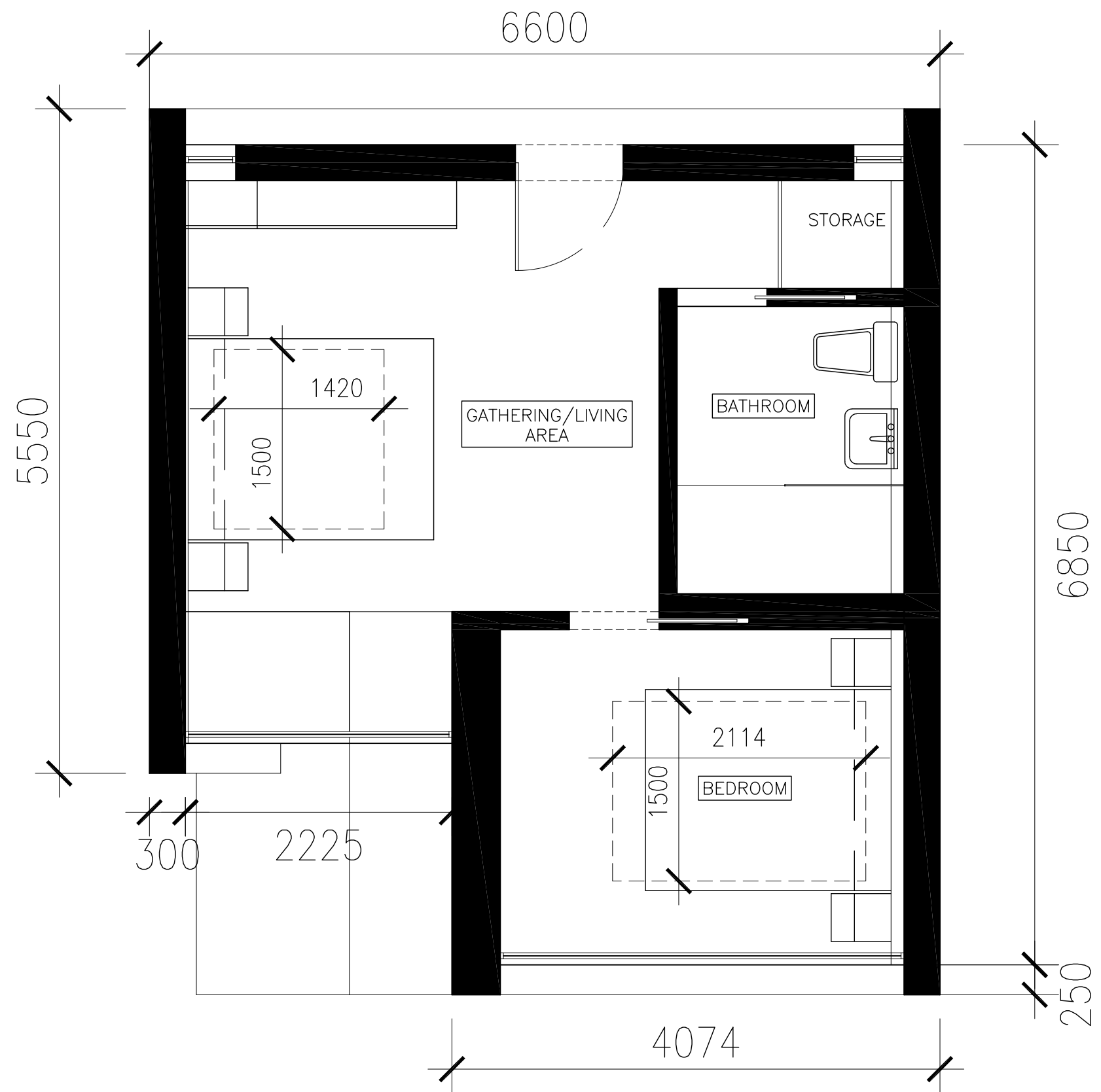
AURORA POD FLOOR PLAN
