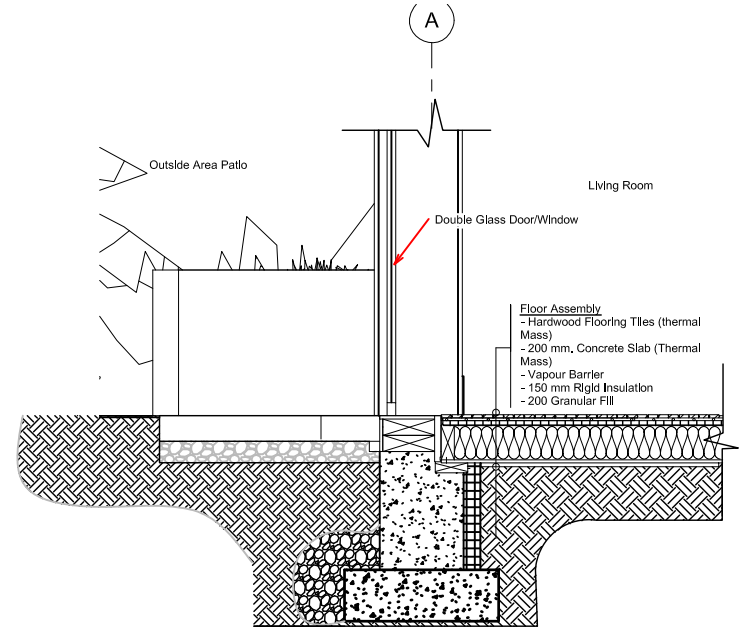
1 DETAIL THERMAL MASS SLAB 1 : 20
