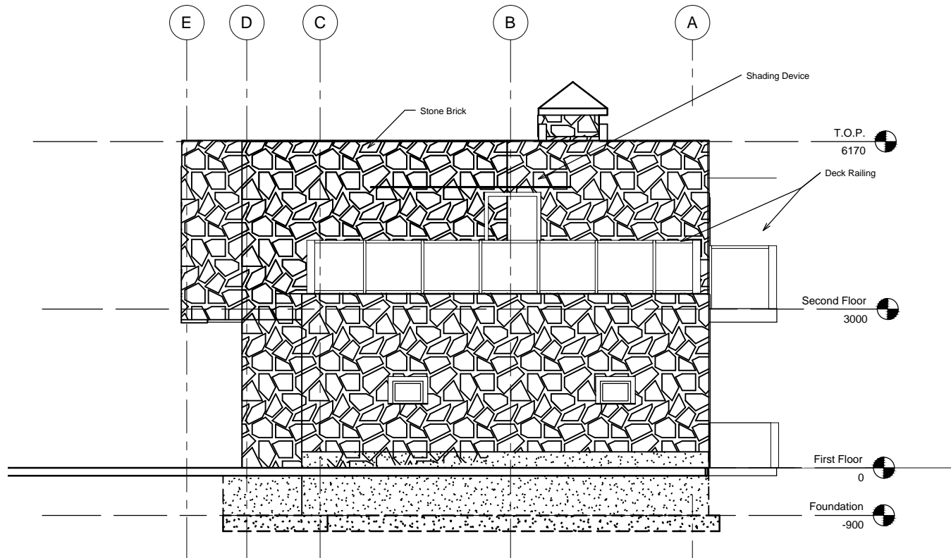
1 East Elevation 1:50
