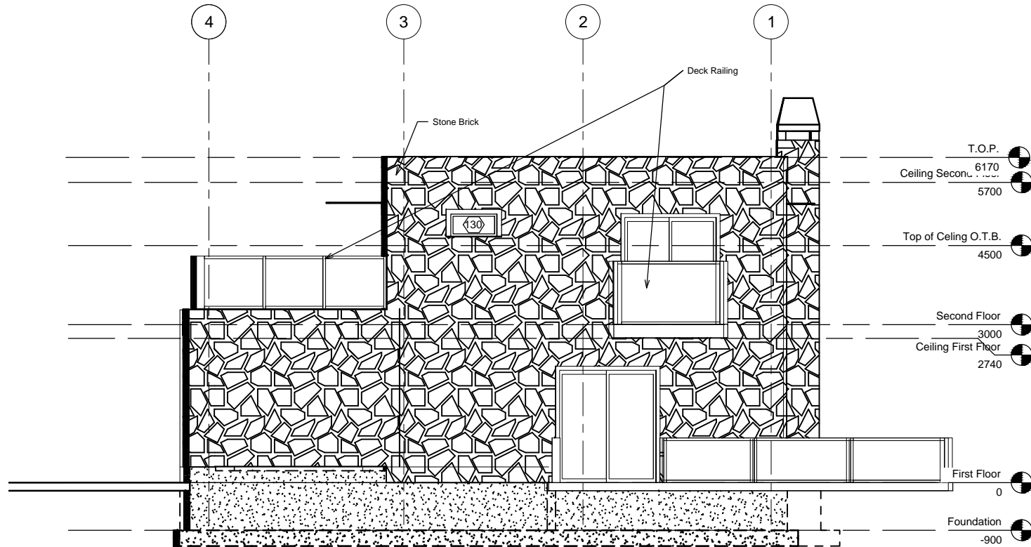
1 North Elevation 1 : 50
