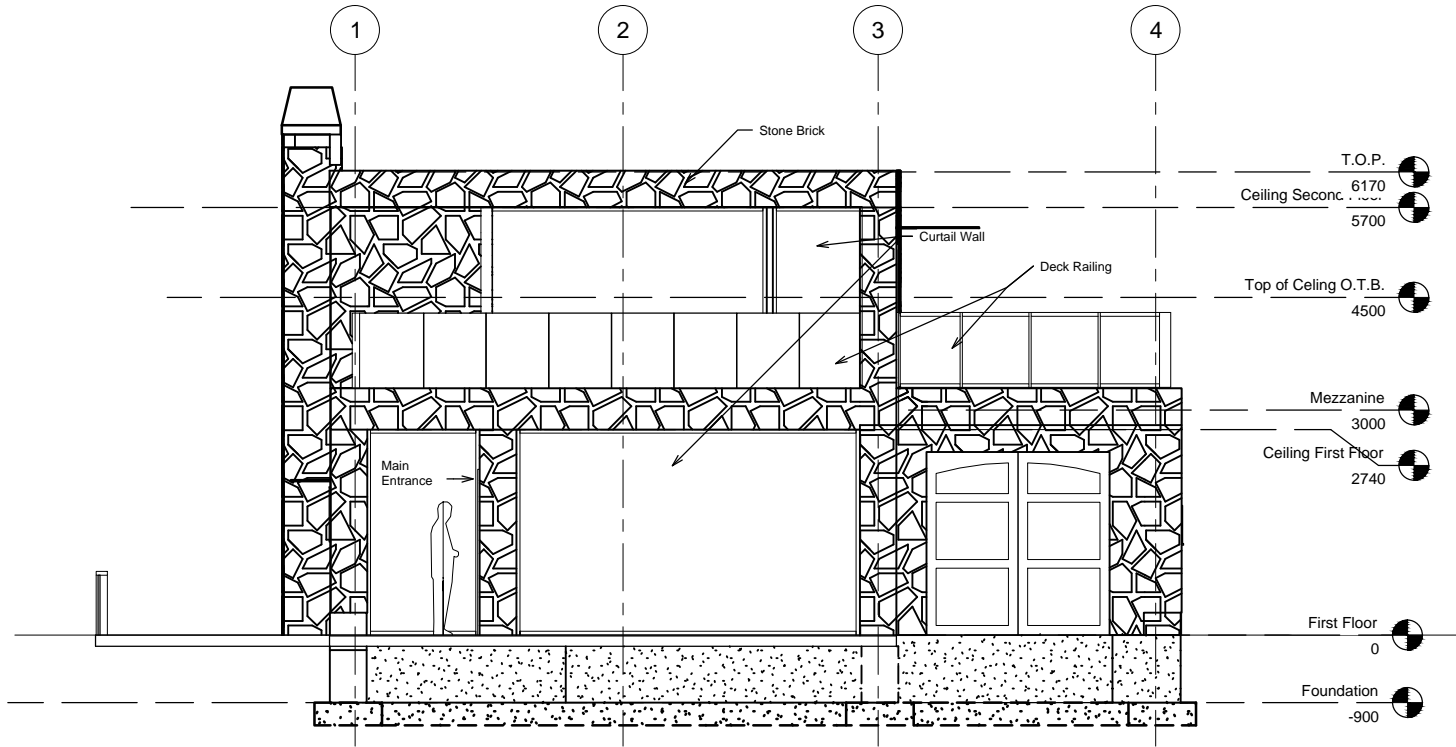
① South Elevation 1 : 50
