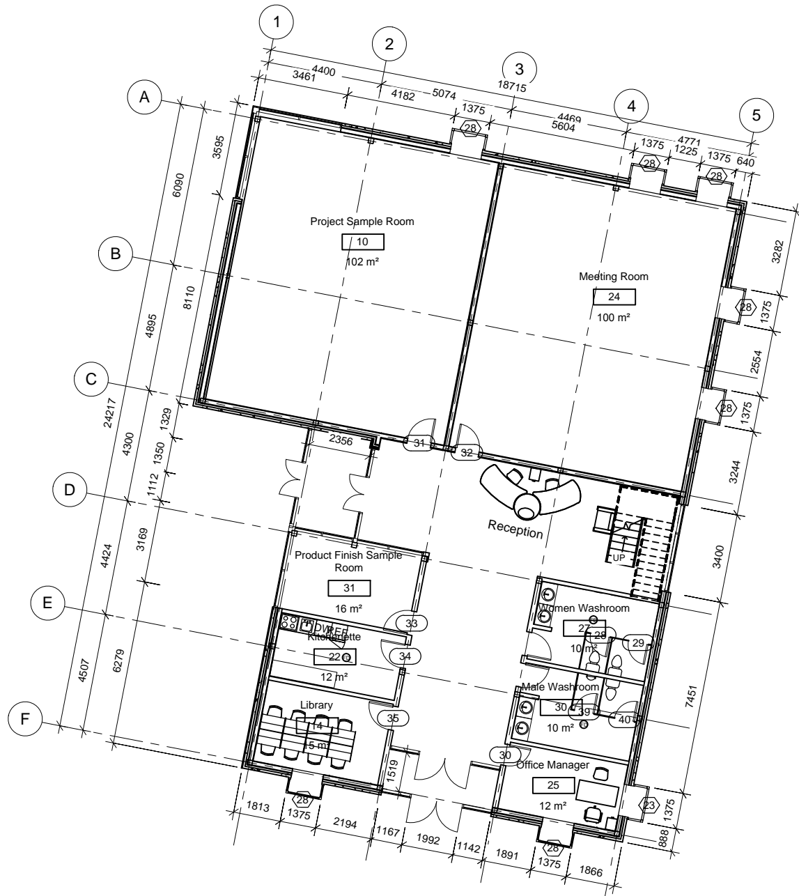
1 FIRST FLOOR 1 : 100
