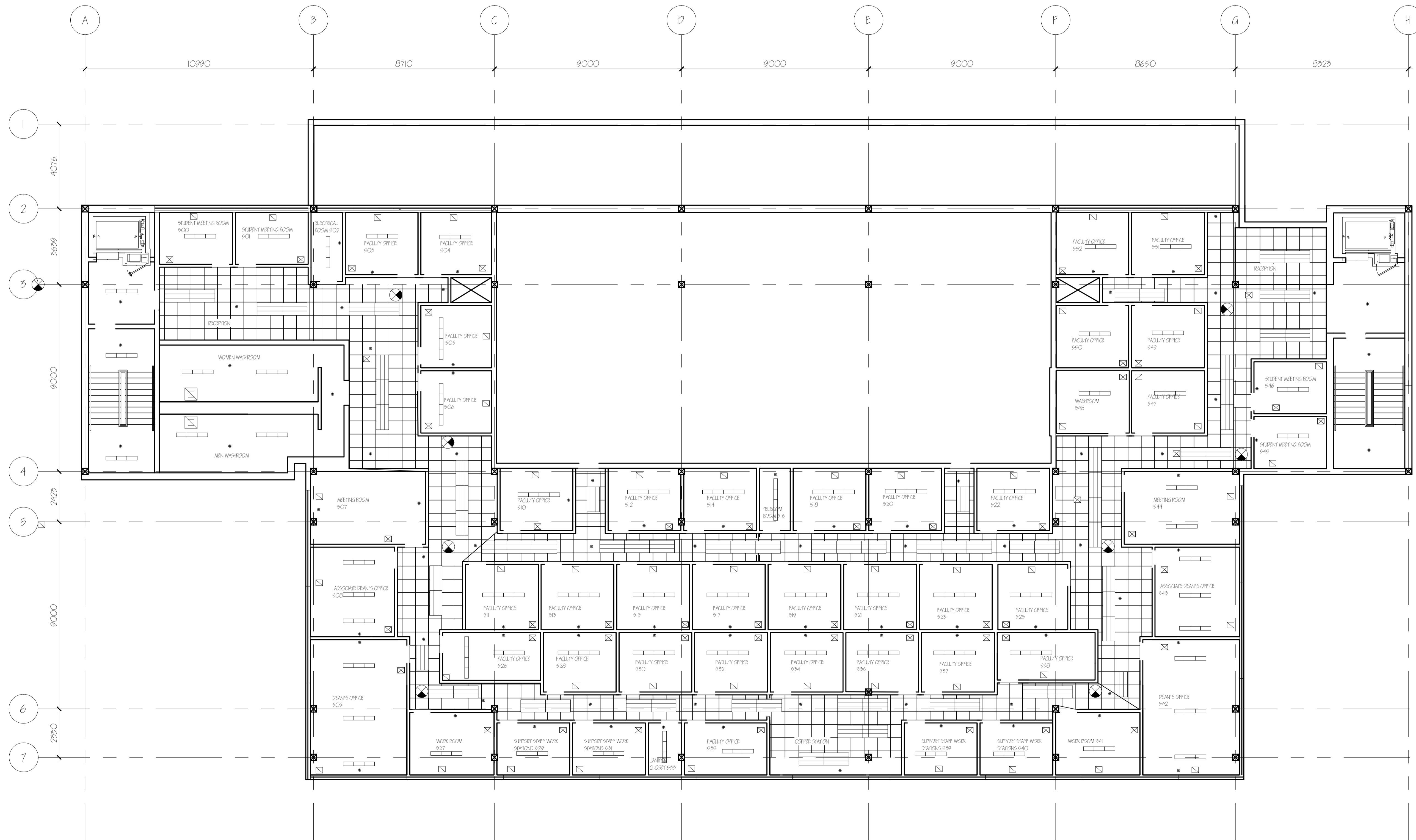
1 500 REFLECTED CEILING PLAN Scale: 1:100
