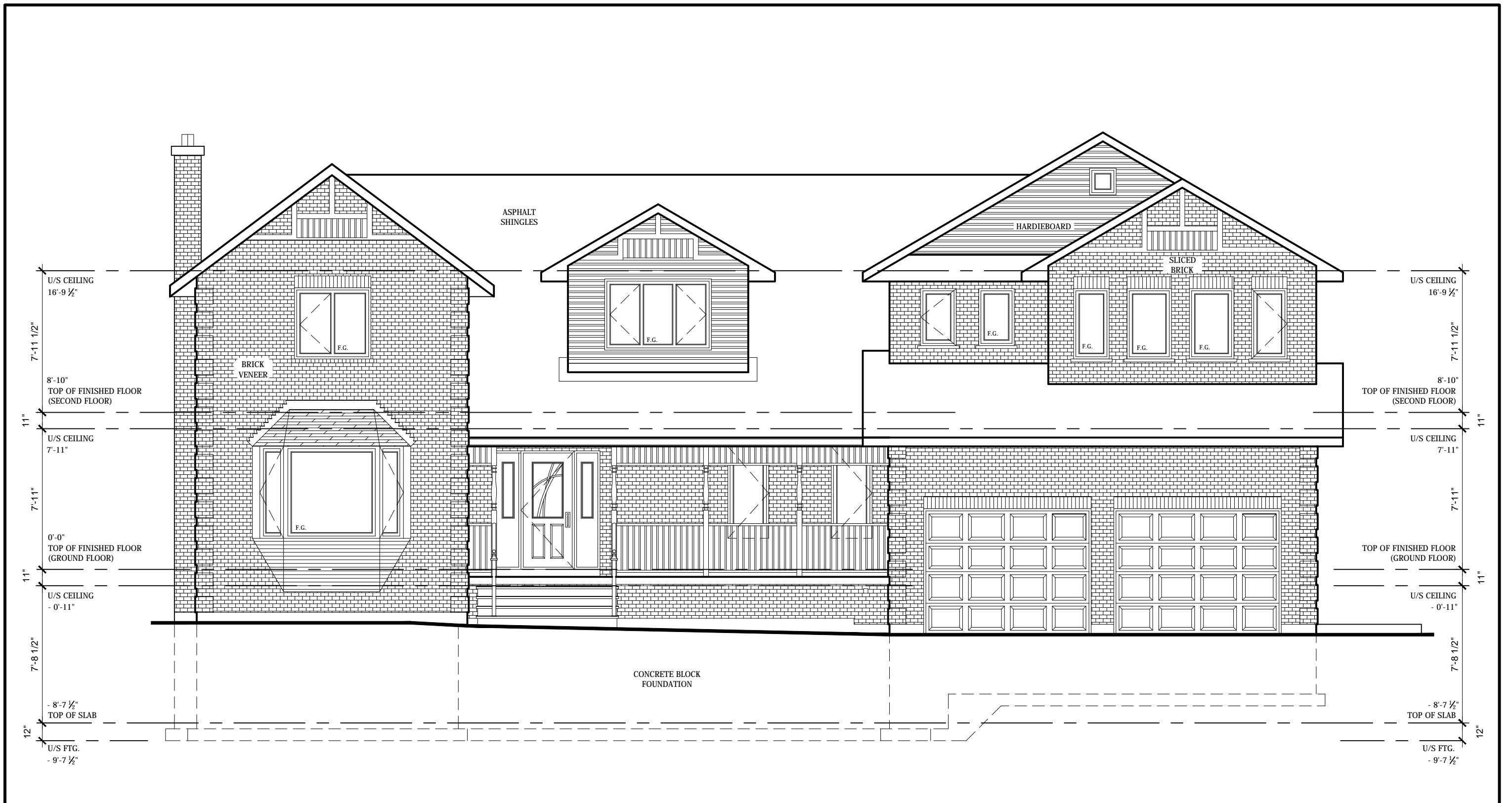
1 EAST ELEVATION Scale: 3/16" = 1'-0"
