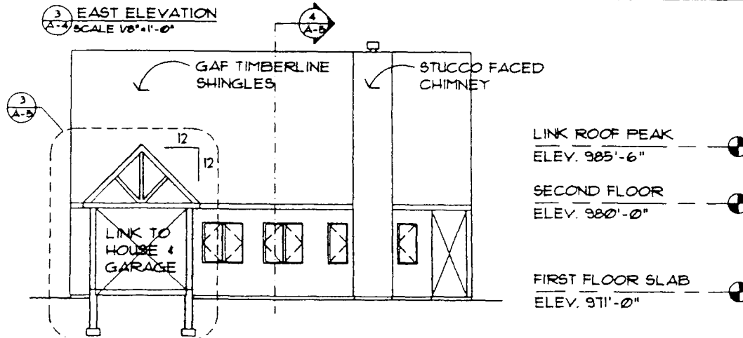
4 NORTH ELEVATION SCALE 1/8" = 1'-0"
