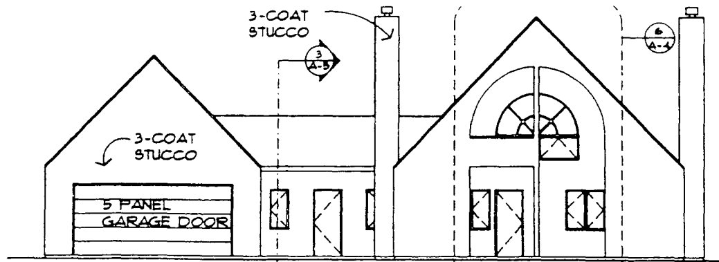
1 WEST ELEVATION SCALE 1/8" = 1'-0"
