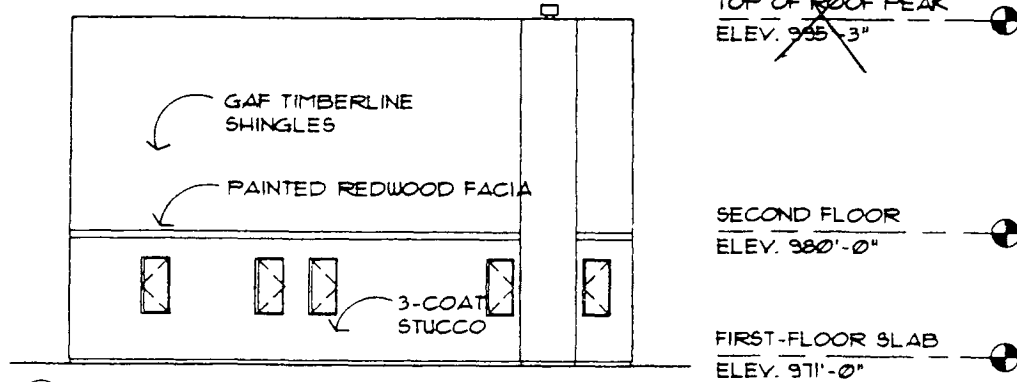
2 SOUTH ELEVATION SCALE 1/8" = 1'-0"
