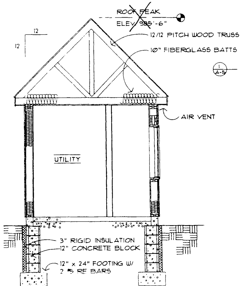
4 SECTION AT HOUSE/GARAGE LINK A-5 SCALE
