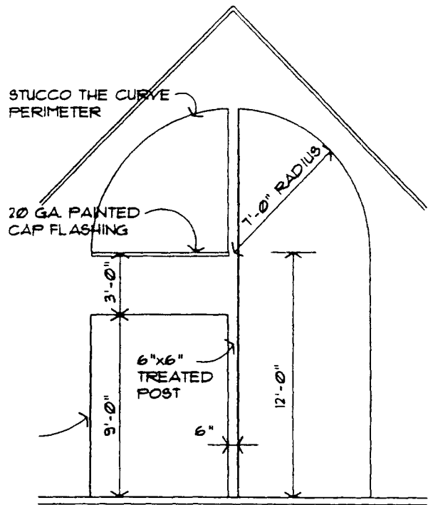
6 WEST ENTRY ELEVATION A-4 SCALE
