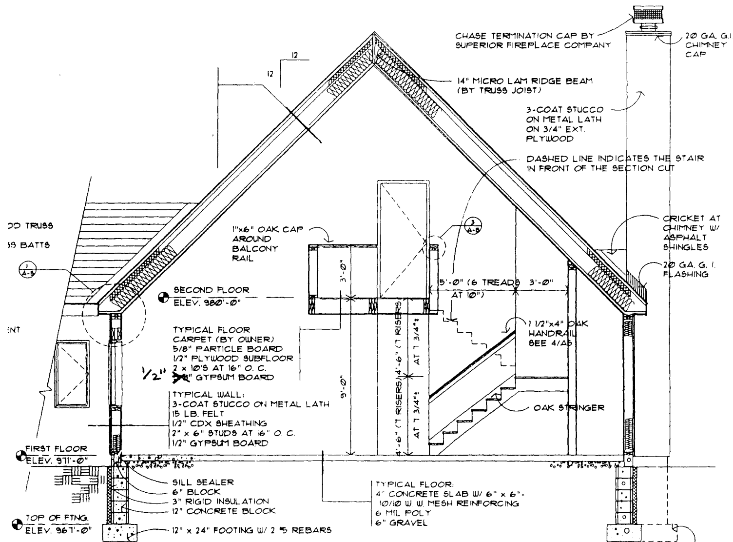
HOUSE SECTION AT STAIR SCALE
