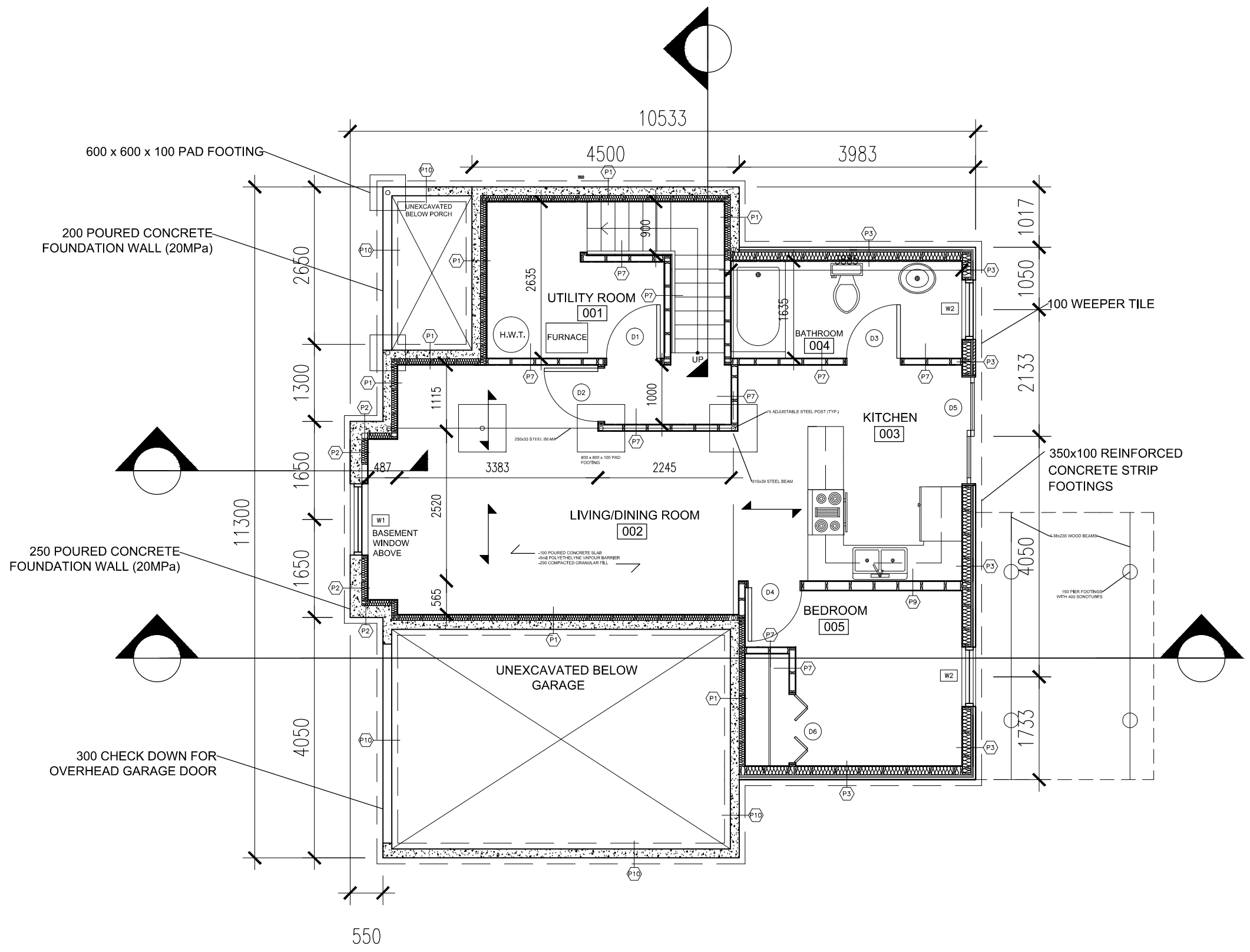
BASEMENT PLAN 1:75
