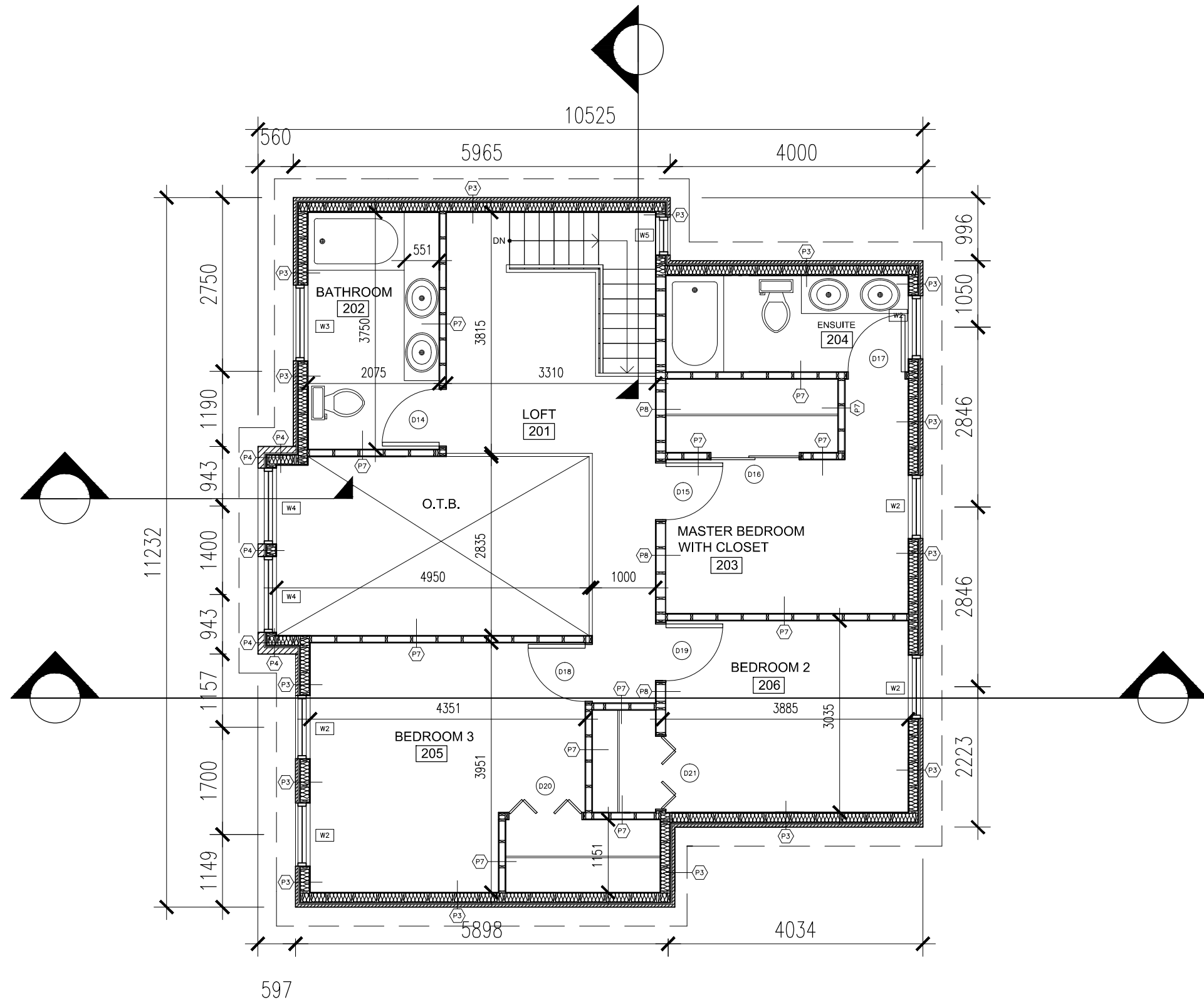
SECOND FLOOR PLAN 1:75
