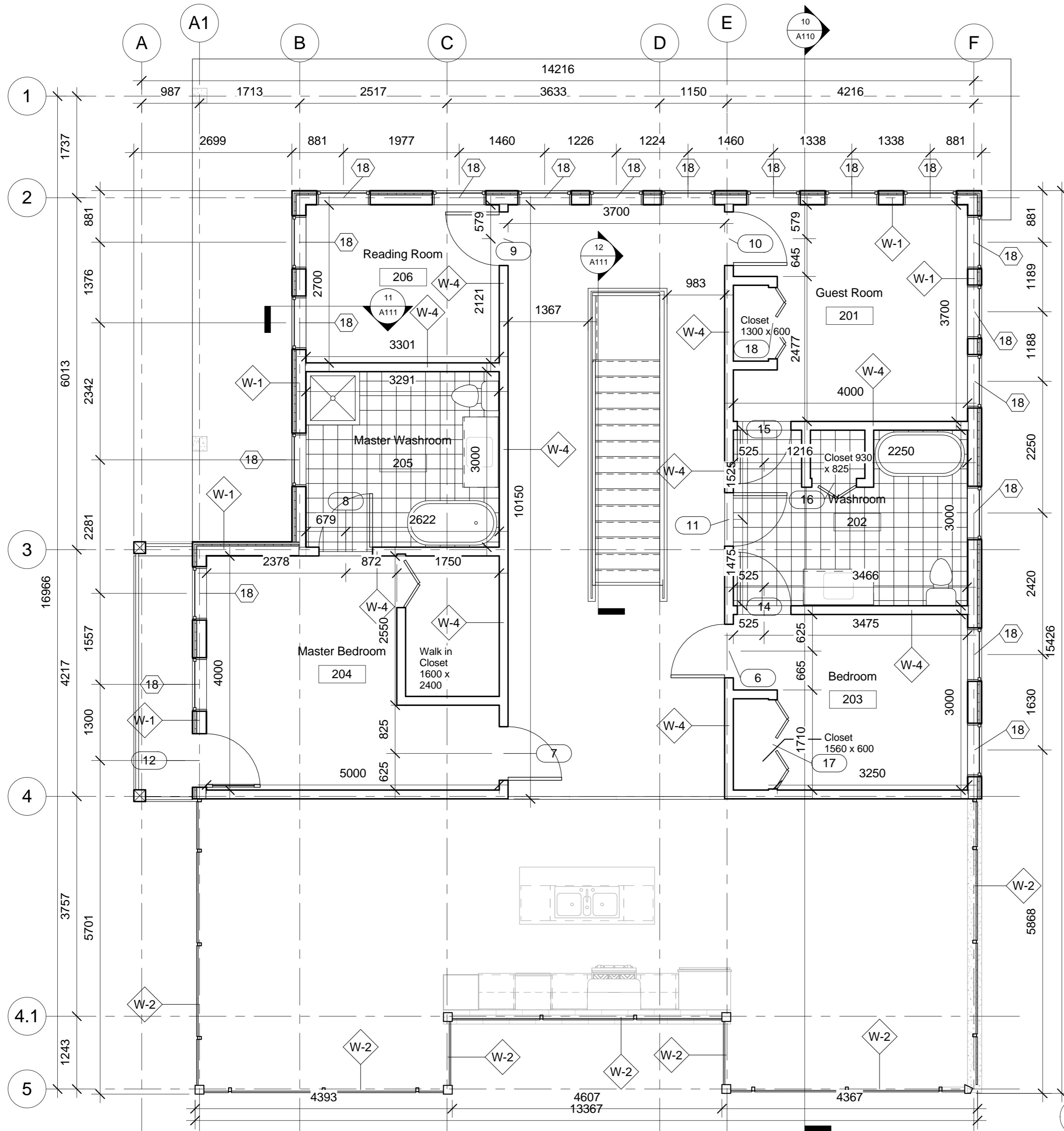
2 2nd Floor 1 : 50
