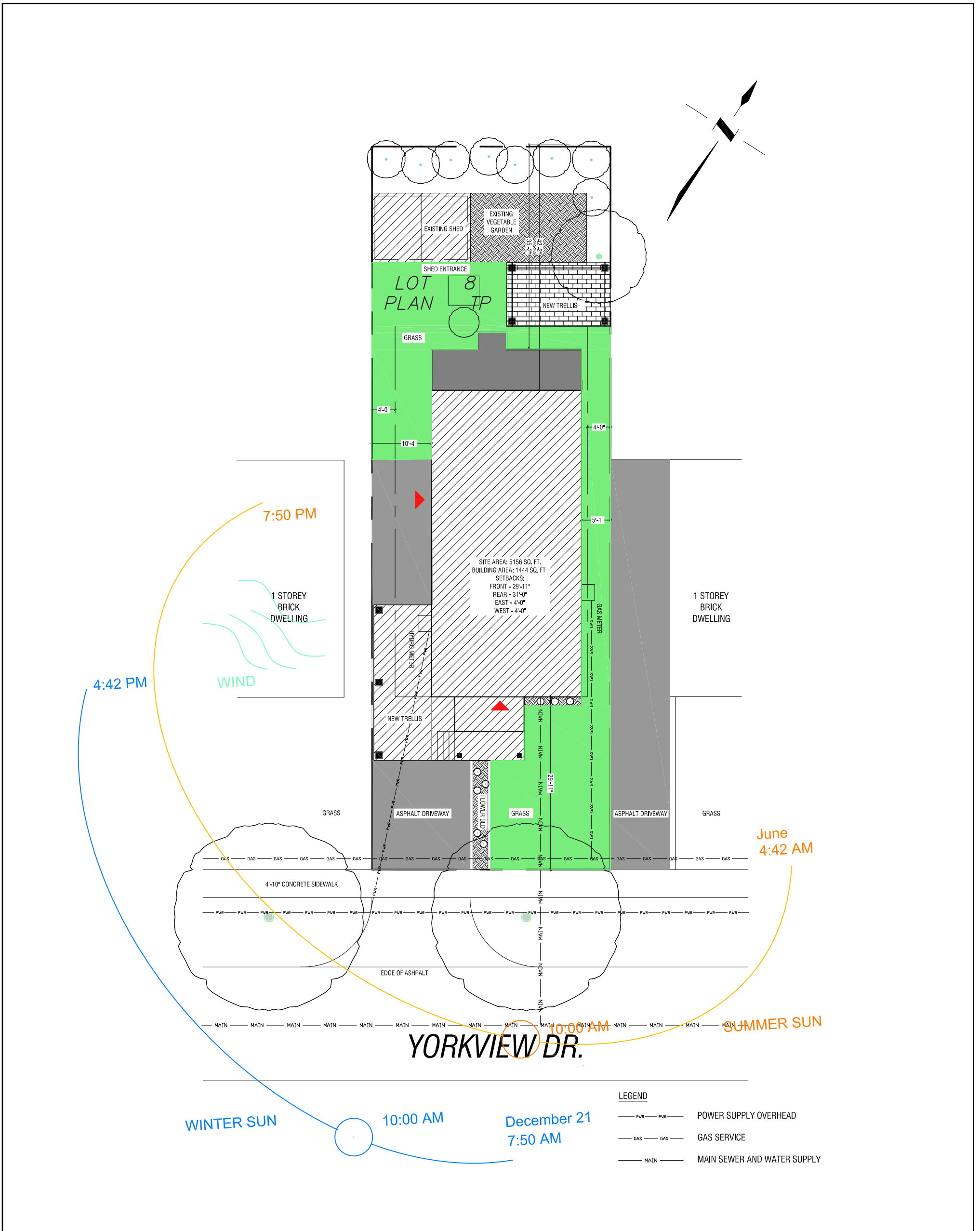
1 PROPOSED SITE PLAN Scale: 1/16" = 1'-0"
