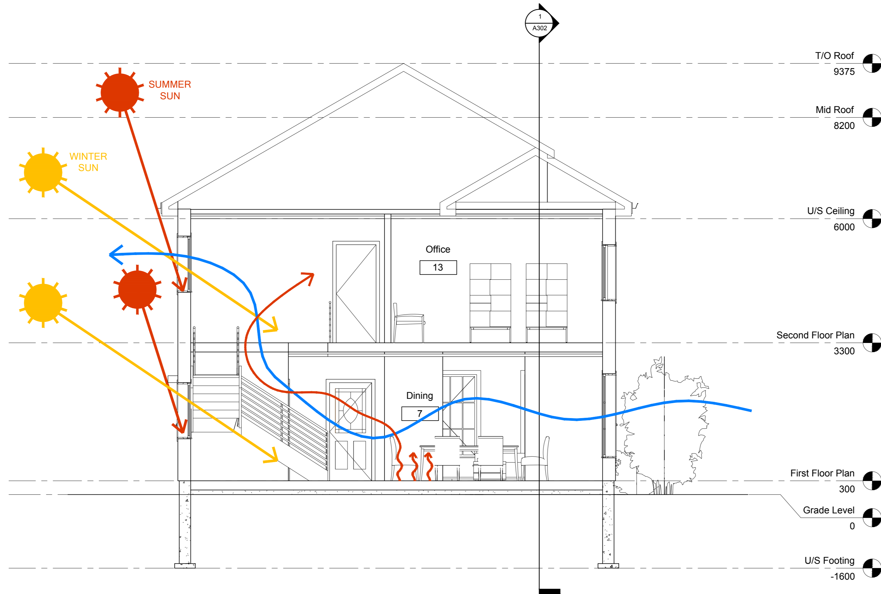
1 N-S Building Section 1 : 50
