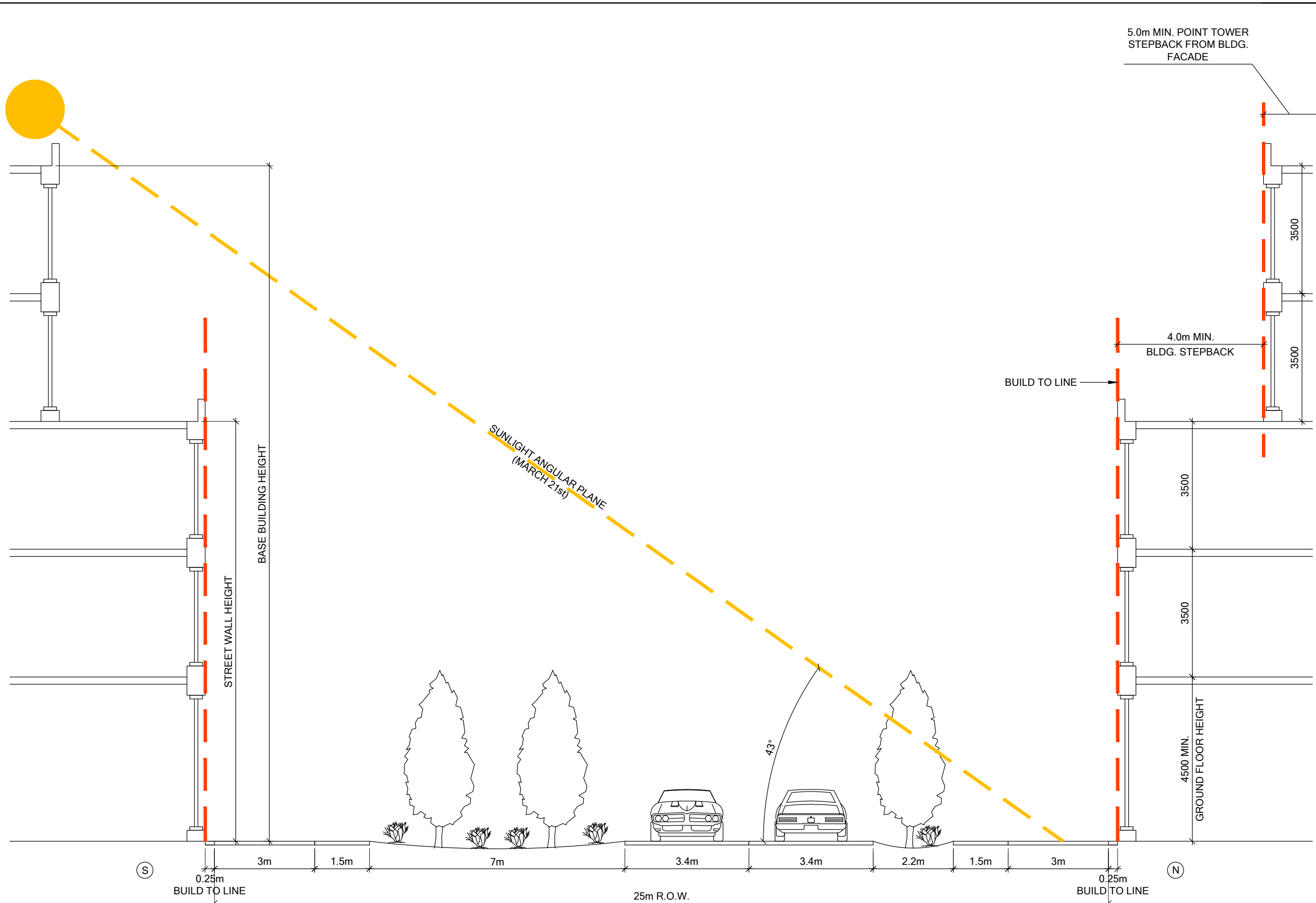
1 STREET SECTION (CITY CENTRE DR. - GREEN CORRIDOR) 8 SCALE : 1:100
