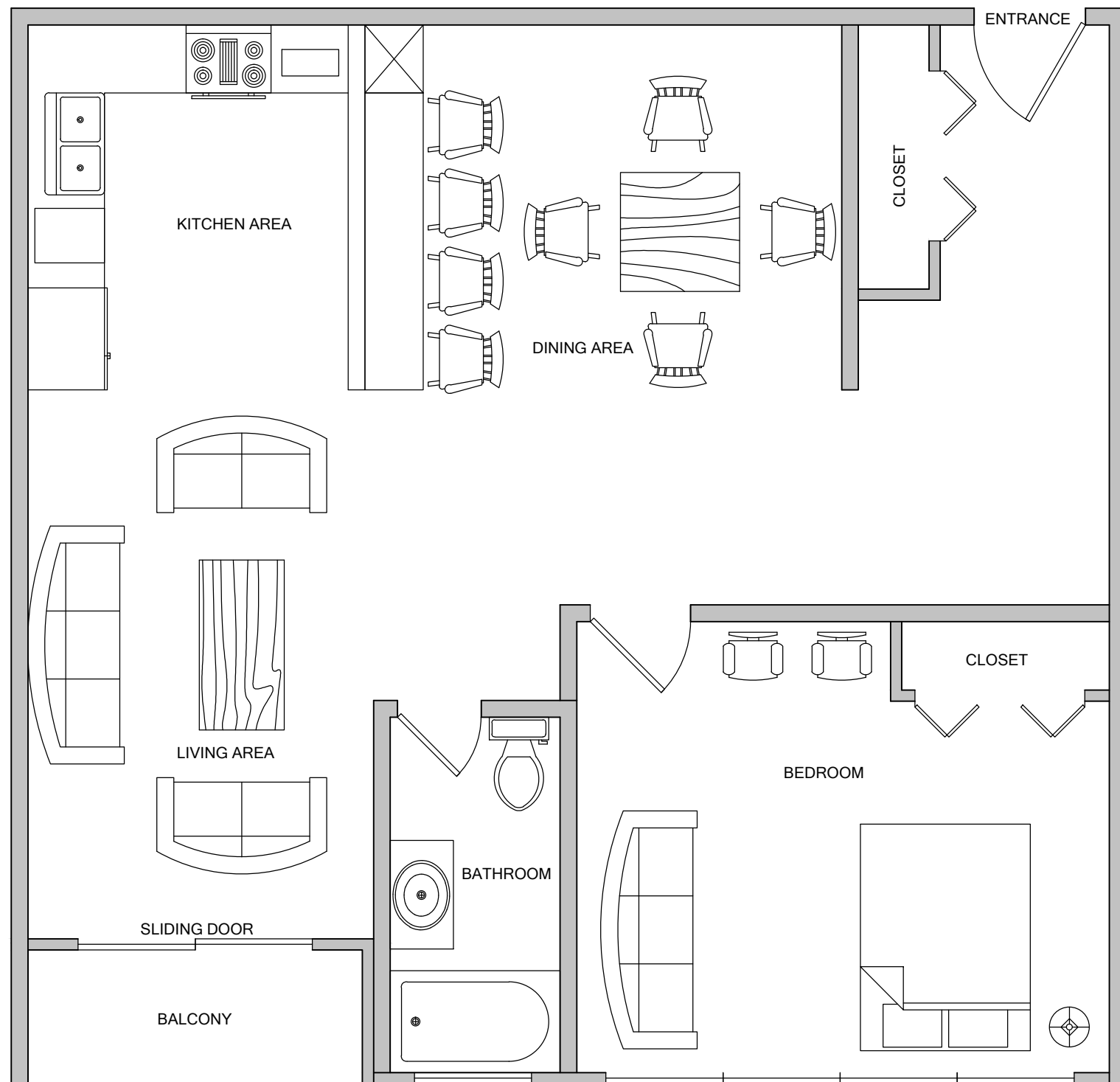
1 TYPICAL UNIT FLOOR PLAN 7 SCALE : 1:50
