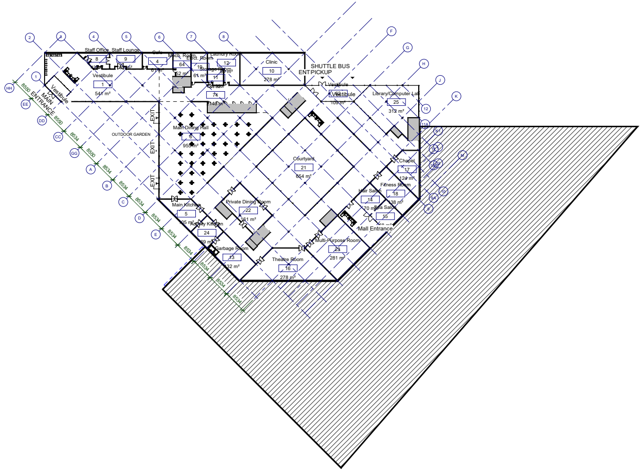
1 Ground Floor 1 : 425
